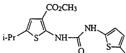
10 5-Isopropyl-2-[3-(5-methyl-thiophen-2-yl)-ureido]-thiophene-3-carboxylic acid methyl ester
